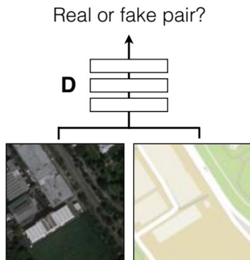
Positive examples
