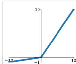
Leaky ReLU
