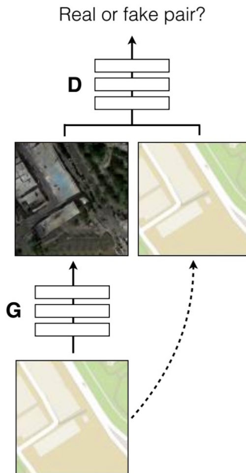
Negative examples
