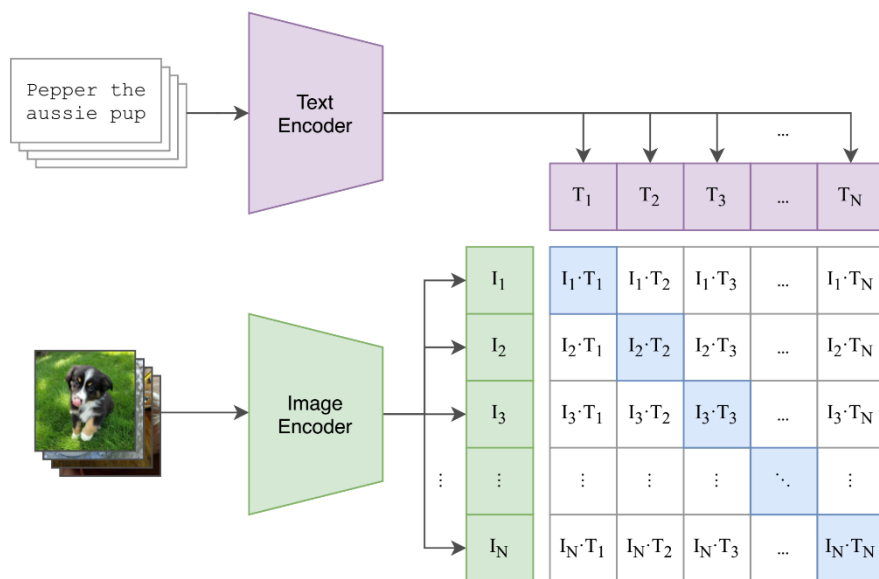
(1) Contrastive pre-training
