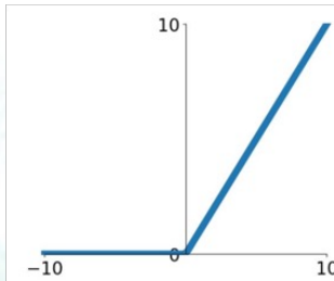
ReLU
